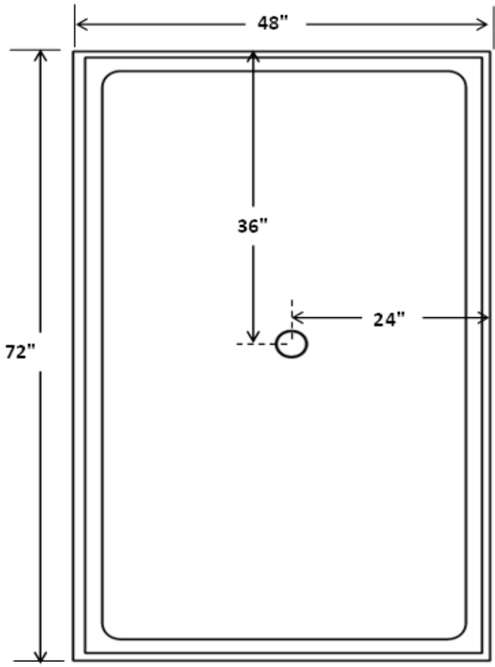
TOP VIEW
